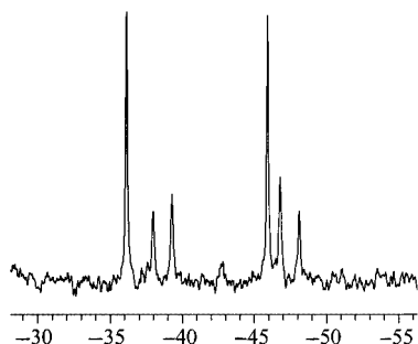
Figure 1. ^{31}\text{P}\{^1\text{H}\} NMR spectrum of the close to statistical mixture of the syn-cis-5c , anti-cis-5c and trans-5c diastereomers (in \text{CD}_2\text{Cl}_2 solution)
