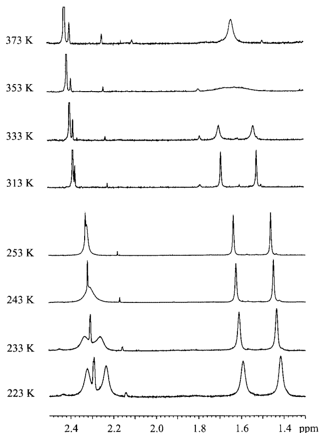
Figure 3. Dynamic ^1\text{H} NMR spectra of 12a (600 MHz, \text{C}_2\text{D}_2\text{Cl}_4 ) showing the rapid equilibration of the diastereotopic -\text{NMe}_2 methyl resonances (left) followed by a markedly slower diastereotopic signal exchange at the adjacent -\text{CMe}_2- moieties (right)
