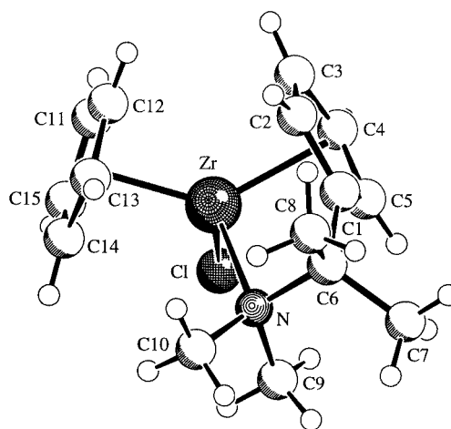
Figure 2. A view of the molecular geometry of 11 in the crystal (only the cation is depicted); selected bond lengths [Å] and angles ^\circ : Zr–N 2.369(3), Zr–Cl 2.426(1), Zr–C 2.398(4) to 2.502(4), C1–C6 1.528(5), C6–N 1.541(5), C6–C7 1.527(6), C6–C8 1.527(6), N–C9 1.491(5), N–C10 1.480(5); N–Zr–Cl 106.0(1), Zr–N–C6 99.6(2), Zr–N–C9 101.0(2), Zr–N–C10 123.5(2), C9–N–C6 112.8(3), C10–N–C6 115.1(4), C9–N–C10 104.2(3), N–C6–C1 100.7(3), N–C6–C7 112.6(3), N–C6–C8 111.0(4), C7–C6–C1 112.7(4), C8–C6–C1 109.8(4), C7–C6–C8 109.7(4)
